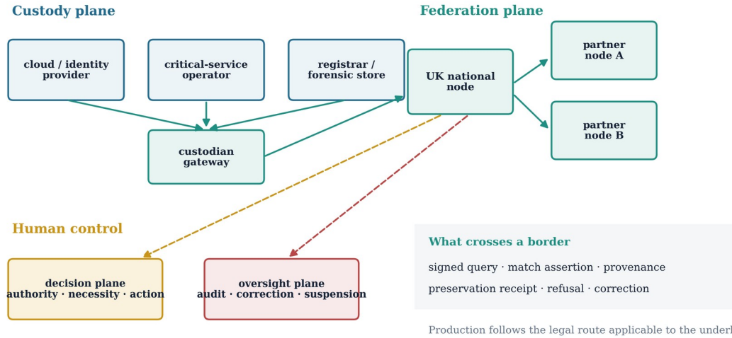
Figure 1. MOSAIC architecture: local evidence custodians connect through national nodes; national nodes federate signed queries; decision and oversight remain outside the automated correlation plane.
